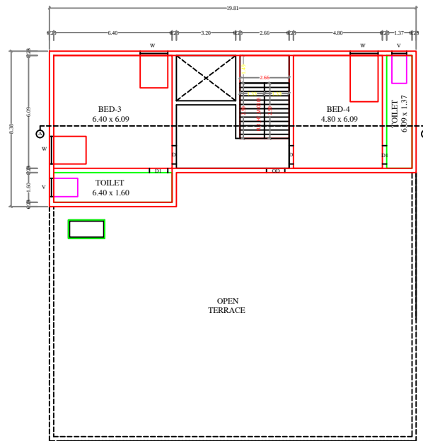
FLOOR-1
