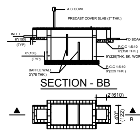
(23) (244) (23) PLAN OF SEPTIC TANK
