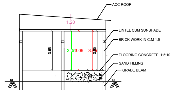
SECTION-AB
