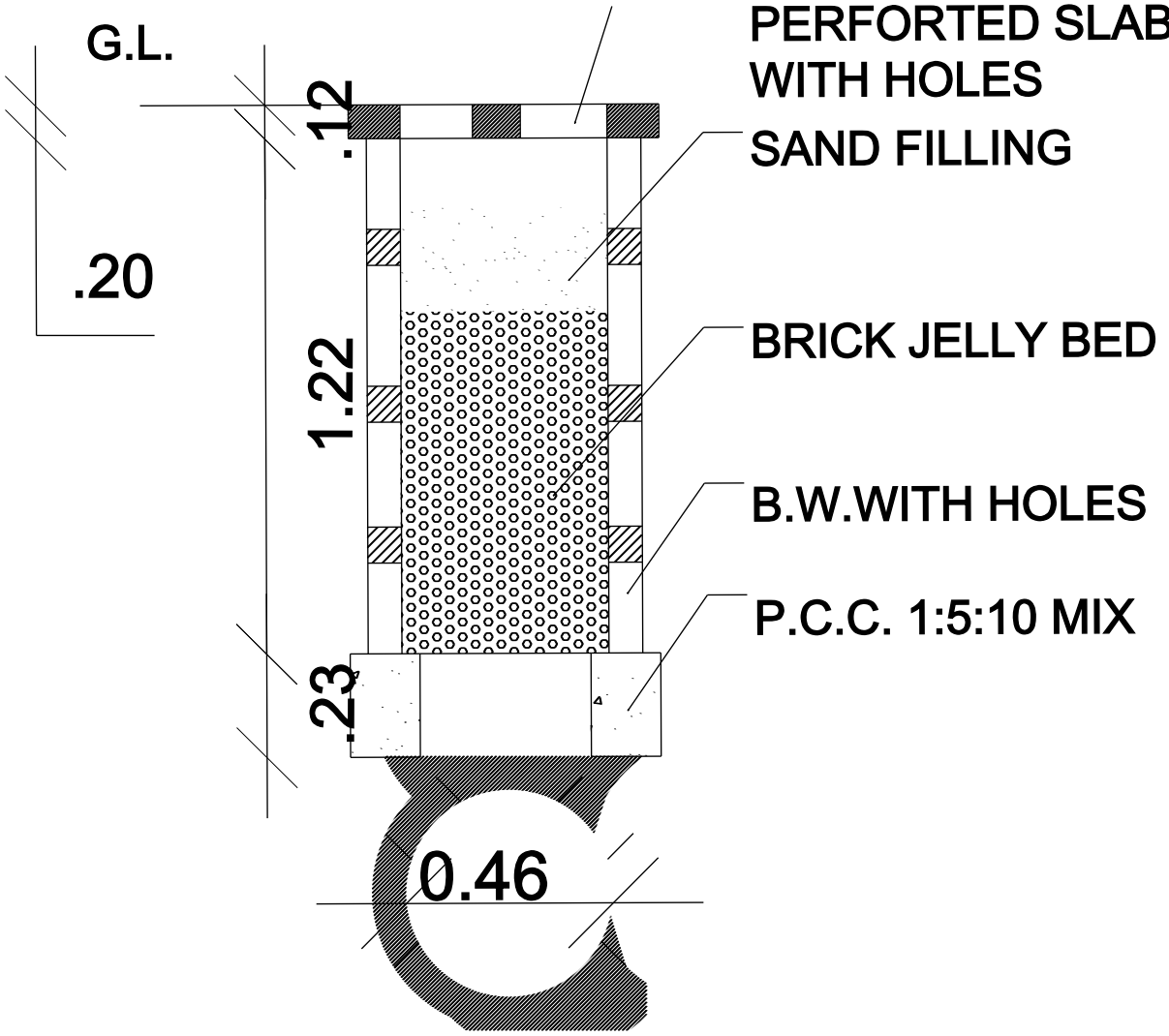
RAIN WATER HARVEST
