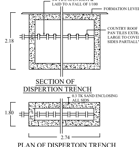
DISPERSION TRENCH
