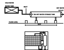
SOLAR HOT WATER SYSTEM DETAILS
