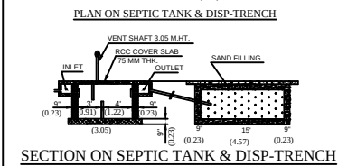
SECTION ON SEPTIC TANK & DISP-TRENCH
