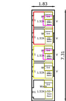
TOILET BLOCK PLAN
