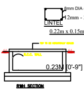
WATER_TANK_CAPACITY_L=2000LTRS
