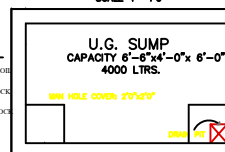
SUMP DETAIL SCALE 1"=4'-0"
