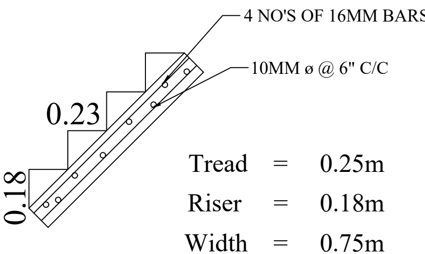
STAIRCASE DETAILS
