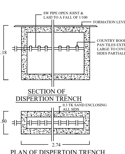
DISPERSION TRENCH
