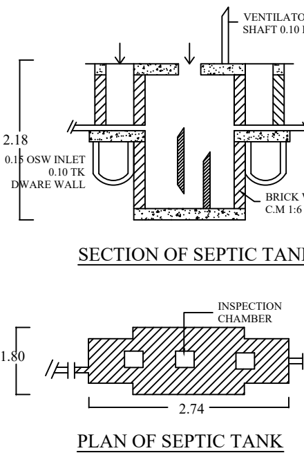
SEPTIC TANK
