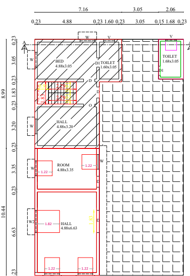
ADDL.FIRST FLOOR PLAN
