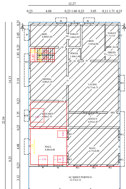
ADDL.GROUND FLOOR PLAN
