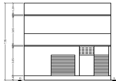
ELEVATION FACING SOUTH
