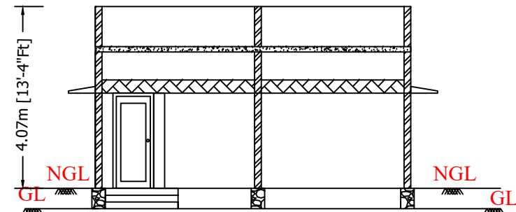
ELEVATION ON NORTH FACE
