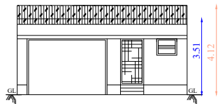
FRONT ELEVATION
