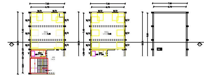
GROUND FLOOR
