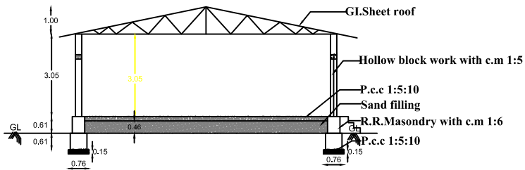
SECTION "XX"
