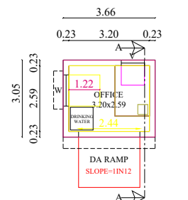
PROPOSED GROUND FLOOR PLAN
