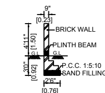
SECTION - CC
