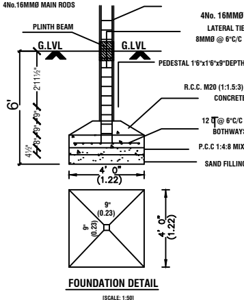
FOUNDATION DETAIL
