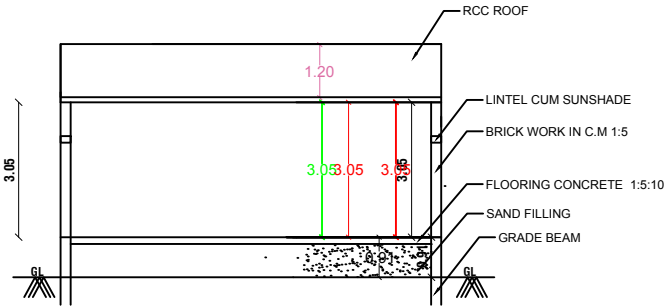
SECTION-AB
