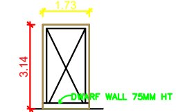
WICKET GATE
