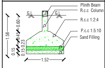
COLUMN FOOTING DETAILS
