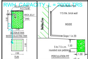
RWH CAPACITY L = 2000 LTRS
