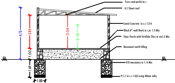
Section on "BC"
