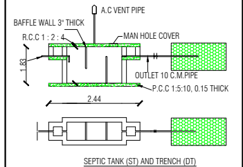
SEPTIC TANK (ST) AND TRENCH (DT)
