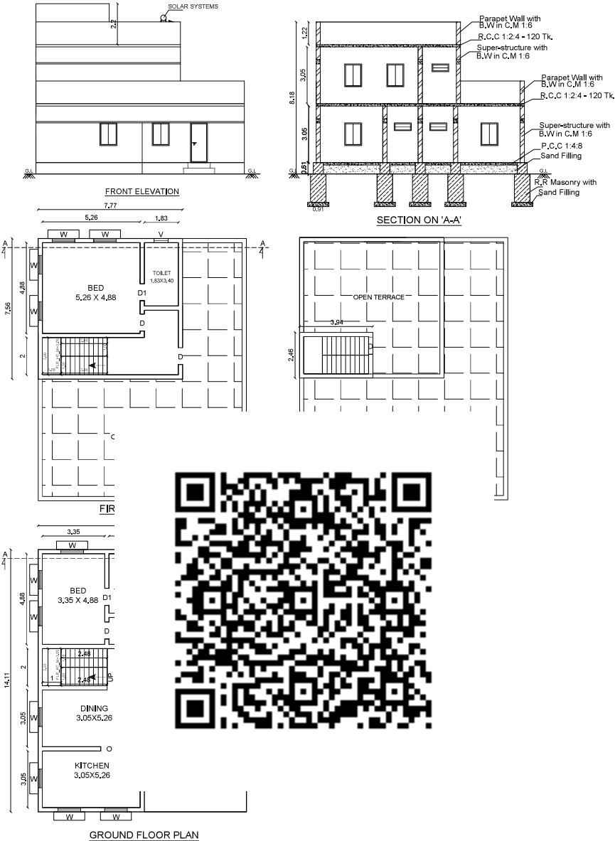
DETAILED PLAN: SCALE 1:100
