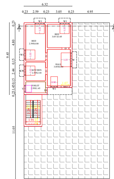
PRO.ADDL.FIRST FLOOR PLAN
