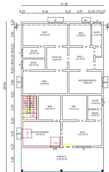
EXT.GROUND FLOOR PLAN
