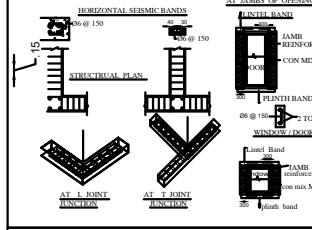
HORIZONTAL SECTION
