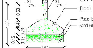
COLUMN FOOTING DETAILS
