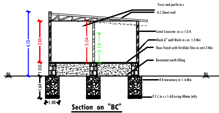
Section on "BC"
