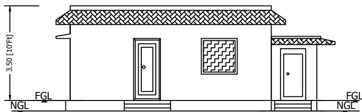
ELEVATION ON EAST FACE
