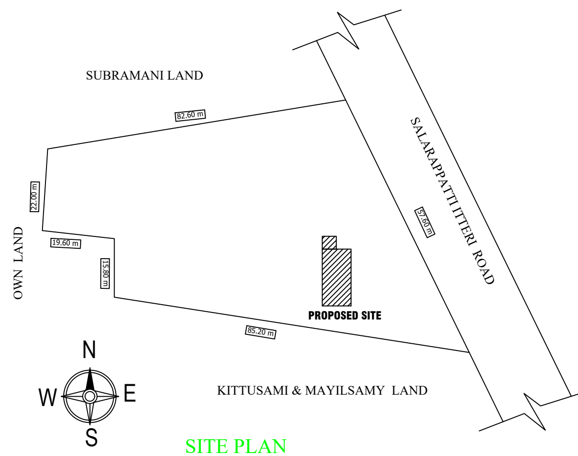
SITE PLAN
