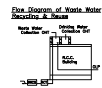
Flow Diagram of Waste Water Recycling & Reuse
