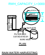
RAIN WATER HARVESTING
