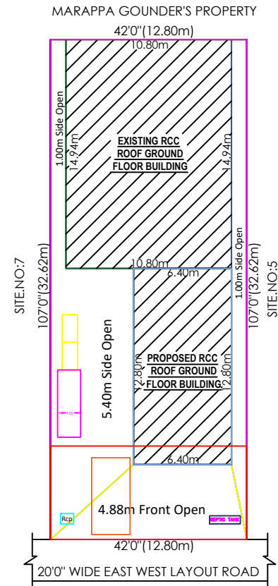
SITE PLAN
