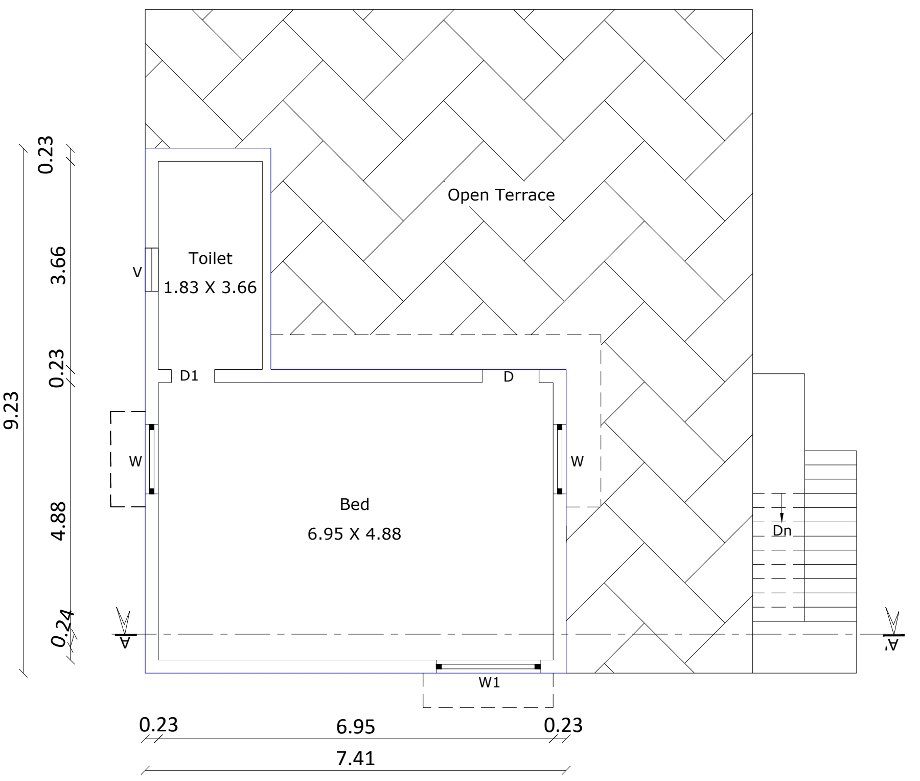
PRO. FIRST FLOOR PLAN
