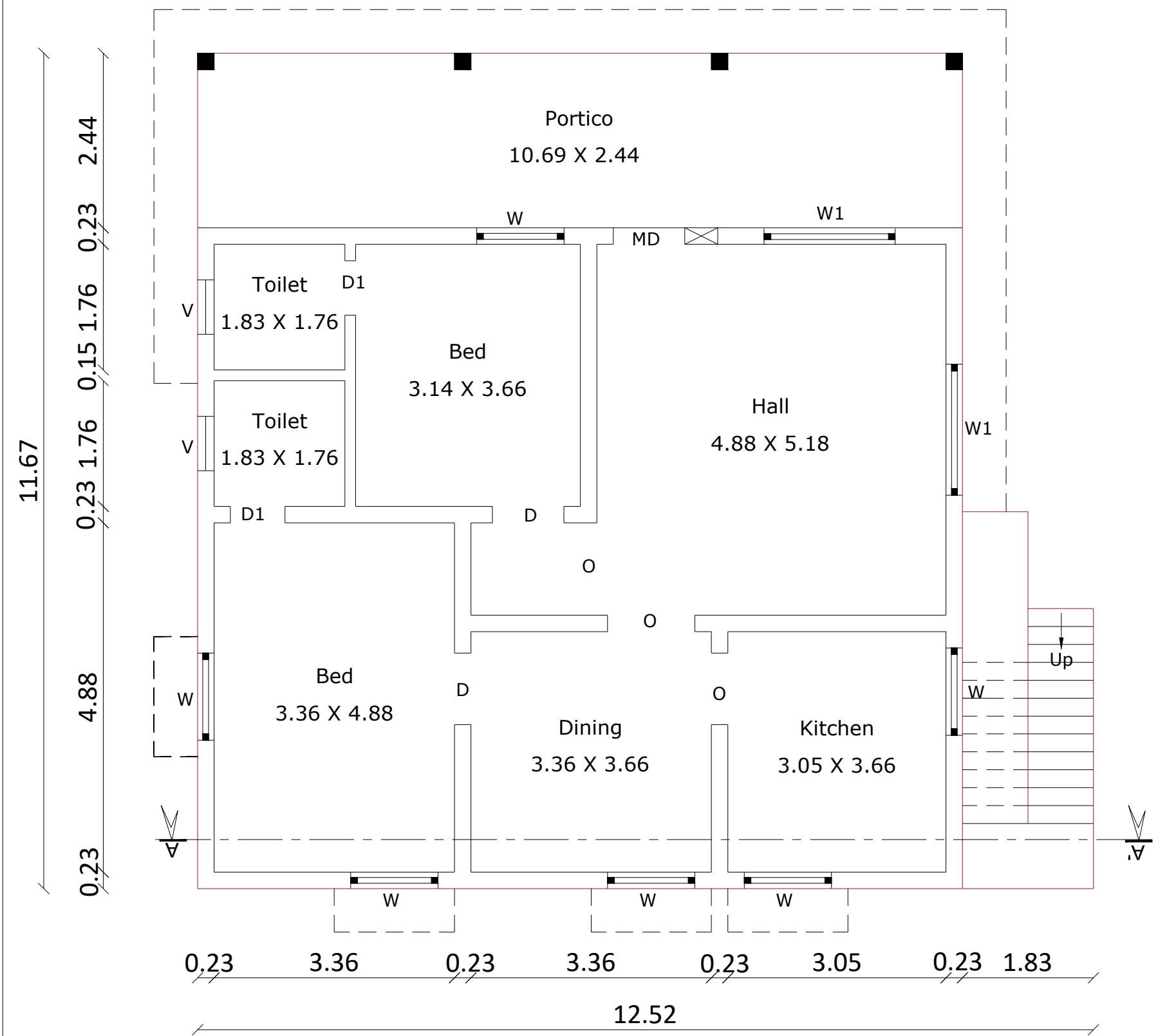
EXI. GROUND FLOOR PLAN
