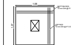
FOOTING PLATE
