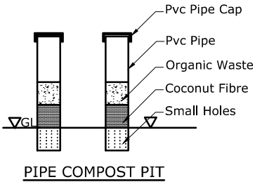
PIPE COMPOST PIT
