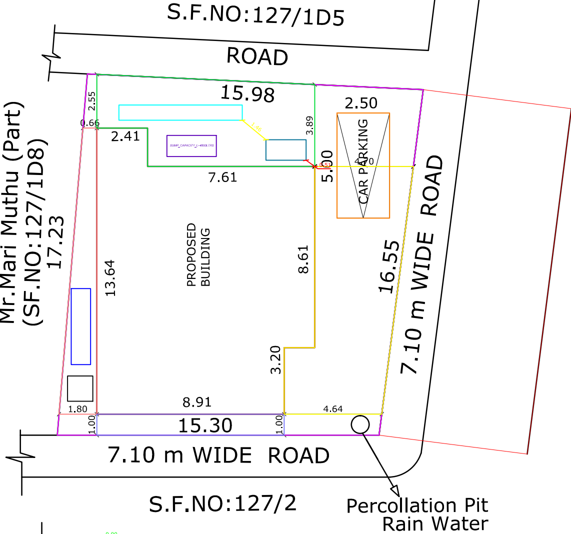
SITE PLAN
