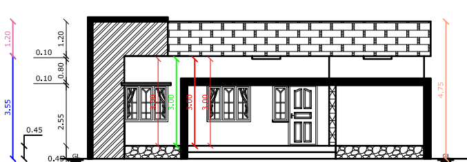
FRONT ELEVATION
