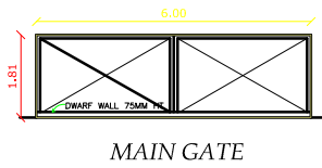
JOINERY DETAILS
