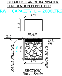
DETAILED PLAN OF RAINWATER PERCOLATION PEBBLE BED
