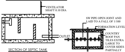
SECTION OF DISPERSION TRENCH
