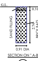
SECTION ON "A-B"
