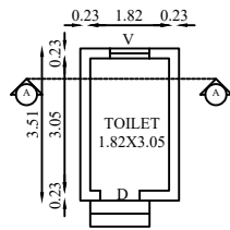
GROUND FLOOR PLAN BLOCK -2
