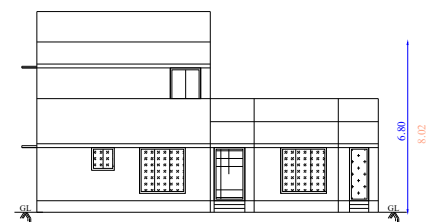
FRONT ELEVATION
