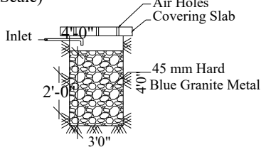
Rain Water Perculation Pit (Not to Scale)
