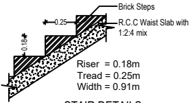
STAIR DETAILS (NOT TO SCALE)
