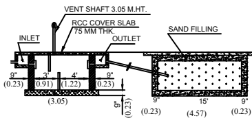
SECTION ON SEPTIC TANK & DISP-TRENCH
