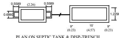
PLAN ON SEPTIC TANK & DISP-TRENCH
