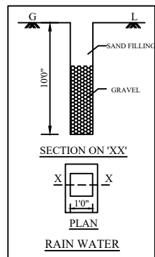
RAINWATER HARVESTING
