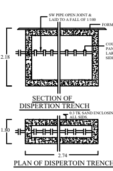
DISPERSION TRENCH
