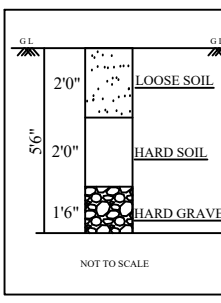
TRIAL PIT
