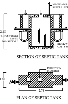
SEPTIC TANK
