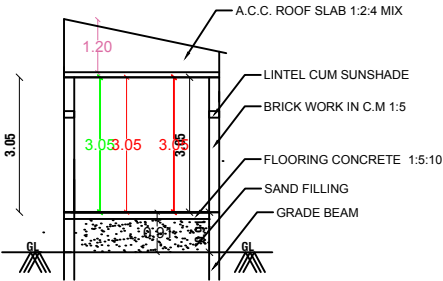
SECTION-AB
