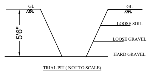
TRIAL PIT (NOT TO SCALE)
