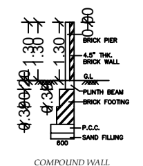
COMPOUND WALL
