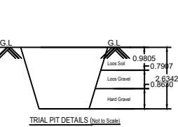
TRIAL PIT DETAILS (Not to Scale)
