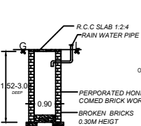
SECTION ON CD
