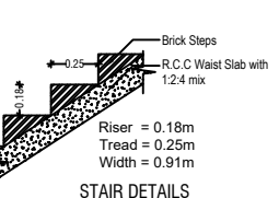
STAIR DETAILS (NOT TO SCALE)
