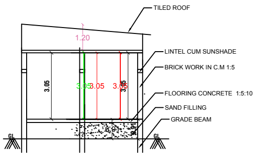
SECTION-AB
