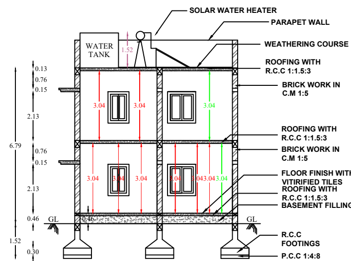
SECTION ON "S S"
