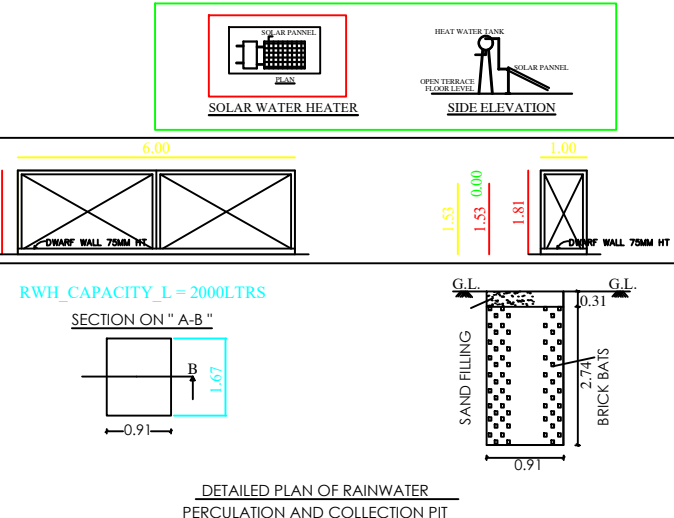
DETAILED PLAN OF RAINWATER PERCUATION AND COLLECTION PIT
