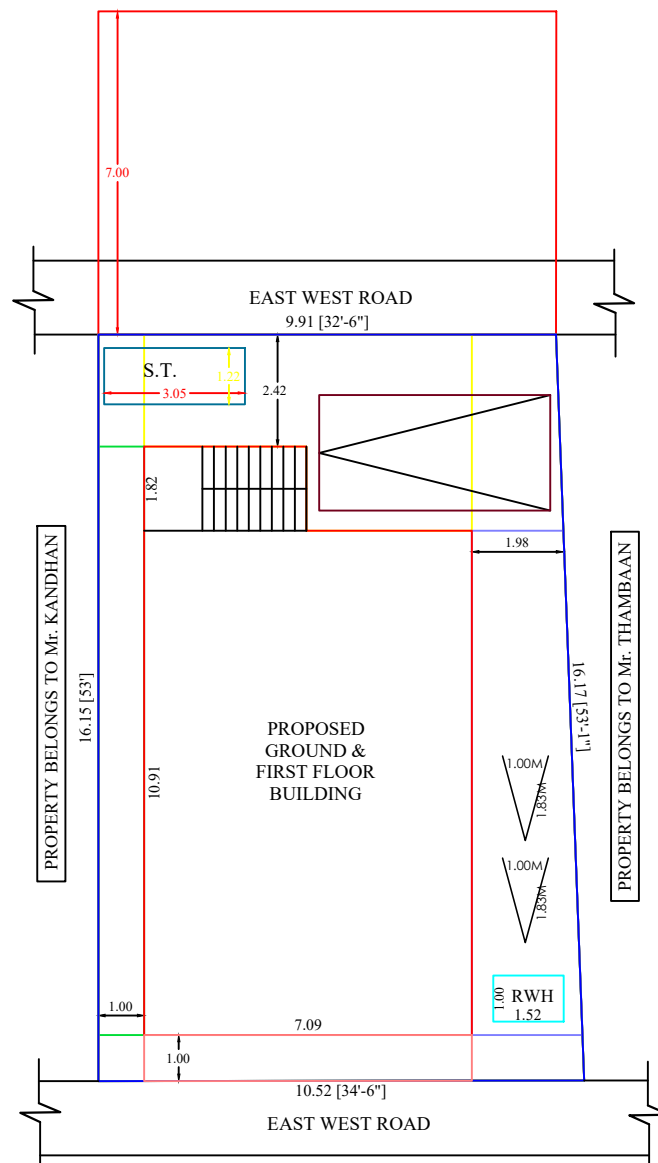
SITE PLAN
