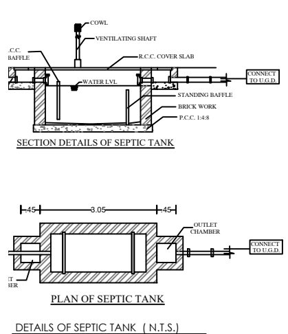
DETAILS OF SEPTIC TANK ( N.T.S )
