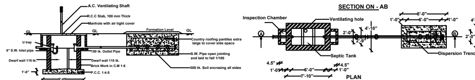
SEPTIC TANK WITH DISPERSION TRENCH ( 250 Gls.,)
