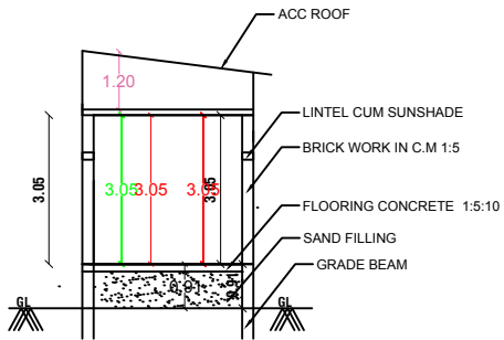
SECTION-AB
