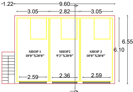
GROUND FLOOR PLAN FACING NORTH
