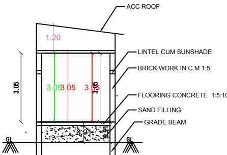
SECTION-AB
