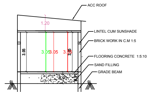
SECTION-AB
