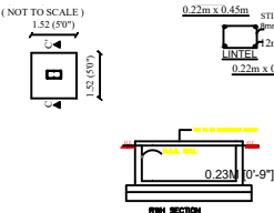
WATER TANK
