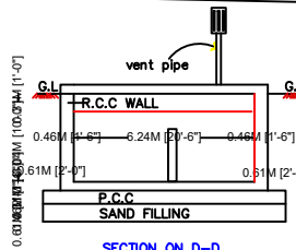
SECTION ON D-D
