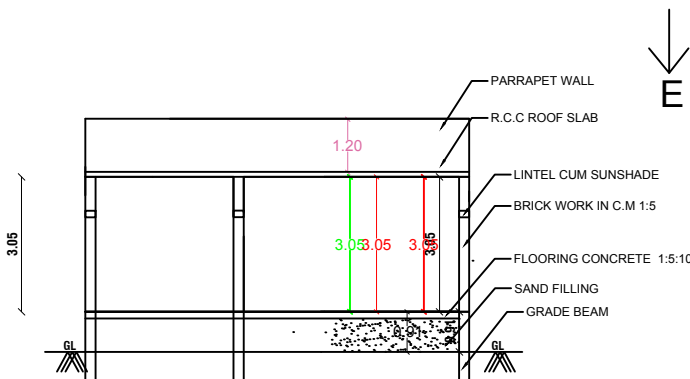
SECTION-AB
