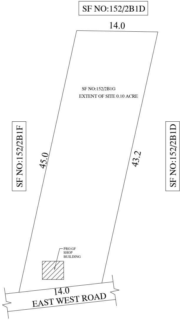
SITE PLAN
