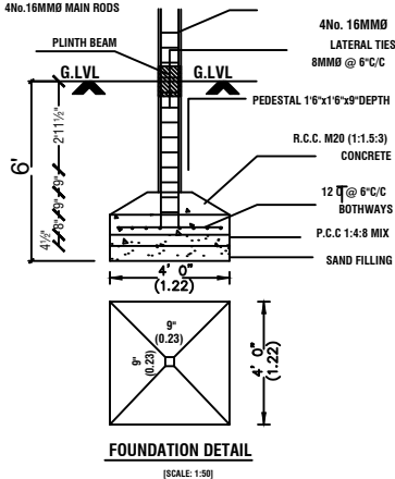
FOUNDATION DETAIL
