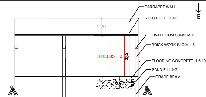
SECTION-AB
