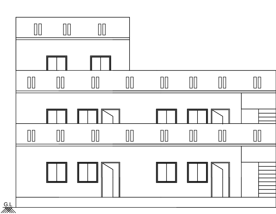
ELEVATION FACING ON EAST
