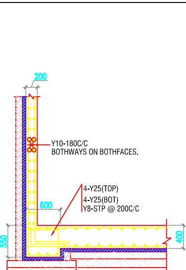
TYPICAL RAFT DETAIL
