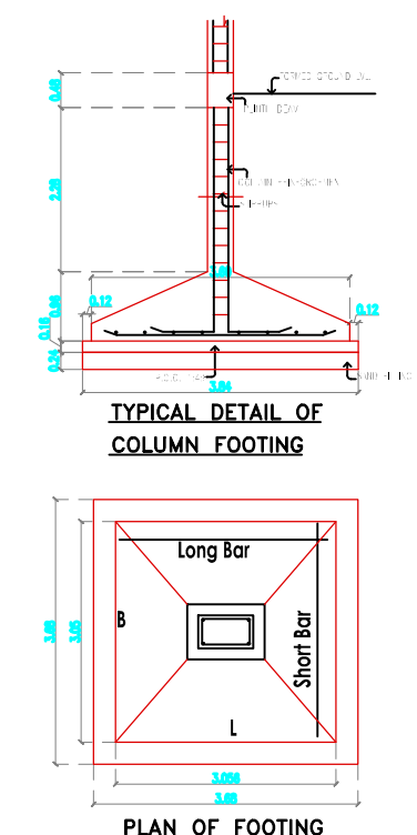
PLAN OF FOOTING
