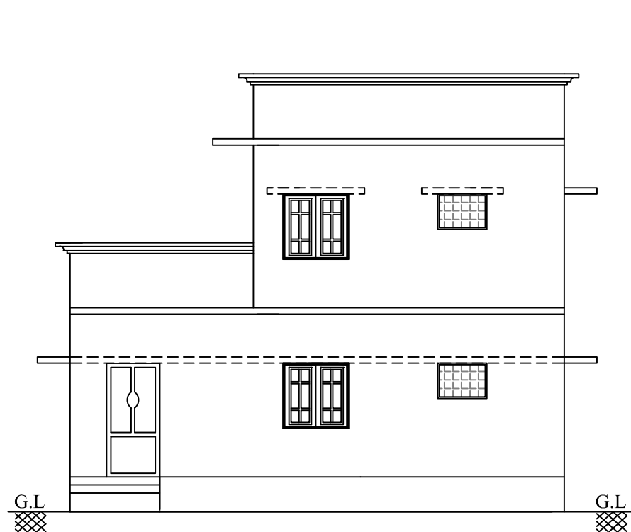
FRONT ELEVATION [FROM NORTH SIDE]
