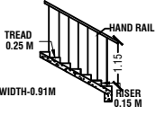
STAIRCASE DETAILS
