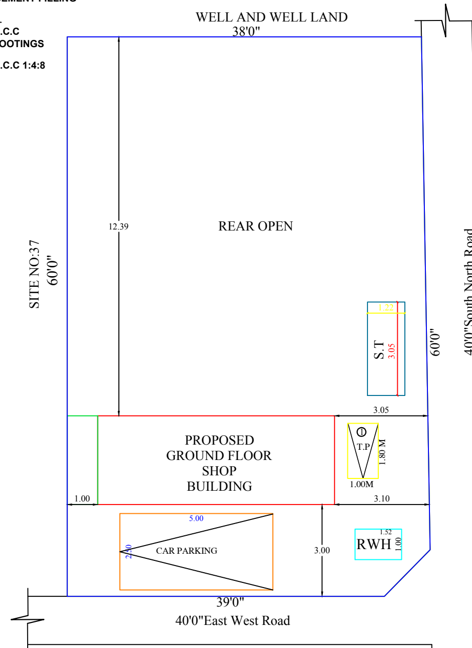
SITE PLAN(1:100)
